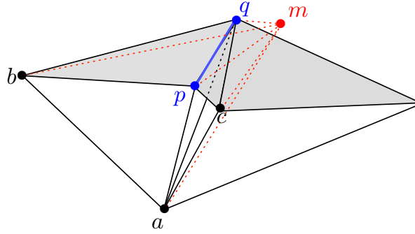
Figure 8.29: Split of boundary edge pq : point m is inserted. Tetrahedron abpq is split into the two valid tetrahedra abpm and abqm , and acqp is split into the two invalid (flipped) tetrahedra acmp and acqm .
