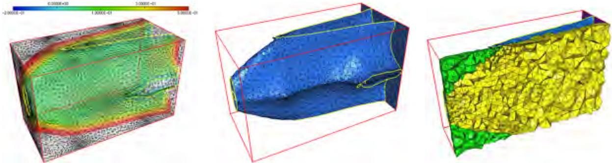
Figure 8.42: (Left): Isosurfaces of the implicit function u on the initial mesh \mathcal{T} , (middle) result of the computation (only the surface mesh \mathcal{I}_{\tilde{\mathcal{T}}} is represented), (right) a cut in the final mesh \tilde{\mathcal{T}} .
