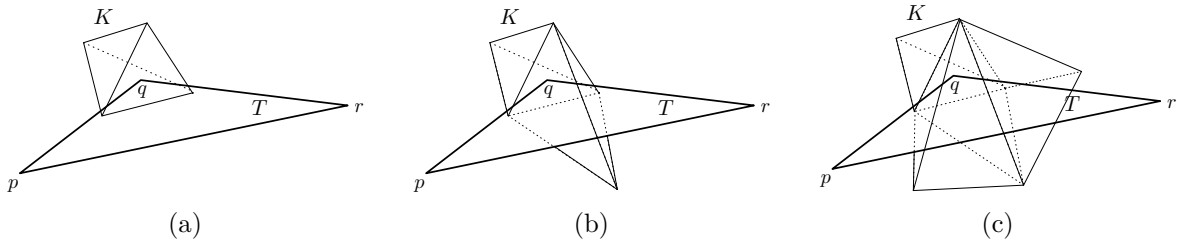
Figure 6.3: Identification of the background simplices intersecting a triangle T = (pqr) \in \mathcal{S} : (a) one starts with a simplex K of \mathcal{T} containing one of the points p, q or r then (b) marches through the faces of K which intersect T and (c) goes on, stopping when there is no more simplex of K to add.
