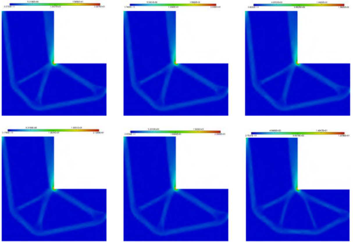
Figure 5.22: (From left to right, top to bottom): stress distribution ( ||\sigma||^2 ) for m = 0, 0.005, 0.01, 0.015, 0.02, 0.05 in the optimal L-Beams displayed on Figure 5.20, using p = 2 .
