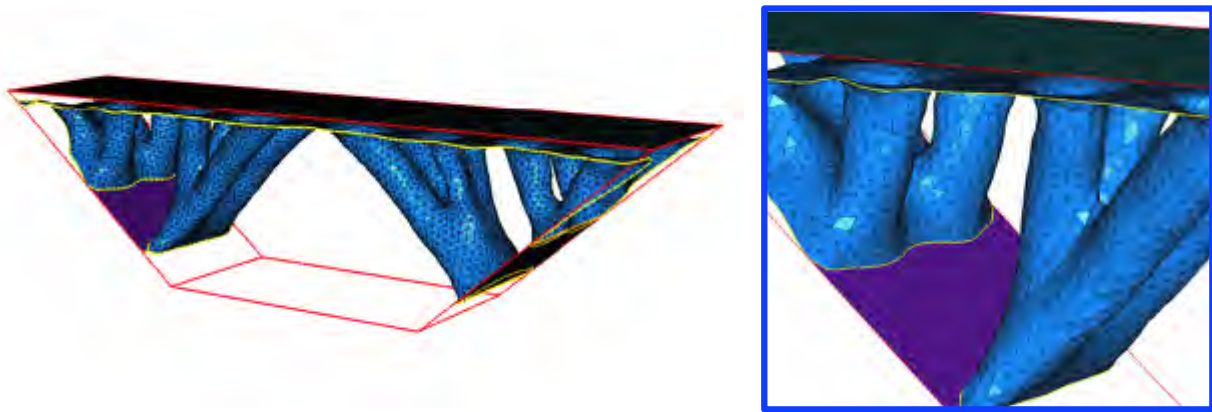
Figure 9.12: (Left) High-resolution mesh of the final shape obtained in the 3d optimal bridge example, (right) zoom on the surface mesh.
