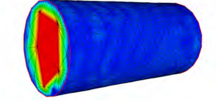
Figure 8.12: Sharp variations of the size map on a cylinder: planar areas may be prescribed an arbitrary large size (displayed in red), while curved areas are more constrained (blue).
