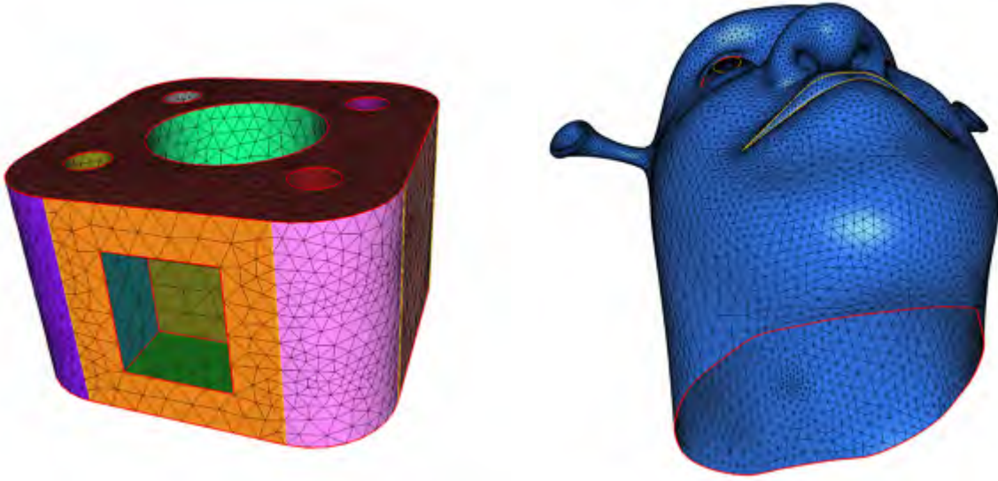
Figure 8.2: ( Left ): Ordinary edges (in black), reference edges (in yellow) and ridges (in red) on a triangulation. Different colors on triangles account for different labels. The points belonging to at least three reference, ridge or required edges are singular points (in green); ( right ): open curve on a triangulation (in red).
