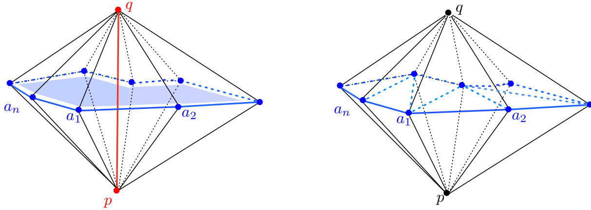
Figure 8.31: Swap of an internal edge pq . (left) The pseudo-polygon associated to the shell \mathcal{Sh}(pq) is enumerated (in light blue), and must be triangulated before being reconnected to p and q (right): one of the many possibilities.
