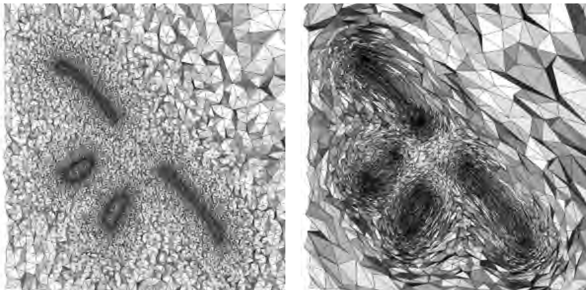
Figure 7.13: (left) A cut in a mesh adapted to the evolving interface at time t = 1.5 using isotropic mesh adaptation ( \approx 1,500,000 points) and (right) anisotropic mesh adaptation ( \approx 700,000 points).
