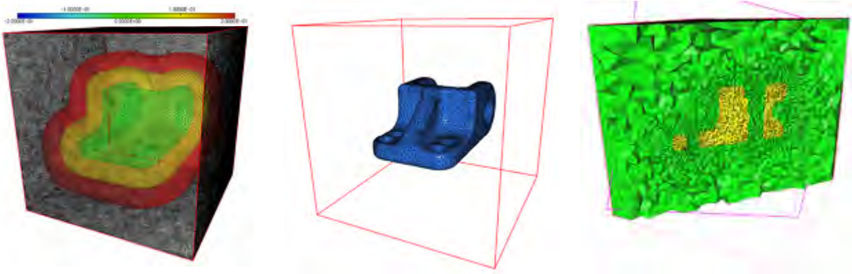
Figure 8.41: (Left): Isosurfaces of the implicit function u on the initial mesh \mathcal{T} , (middle) result of the computation (only the surface mesh \mathcal{I}_{\tilde{\mathcal{T}}} is represented), (right) a cut in the final mesh \tilde{\mathcal{T}} .
