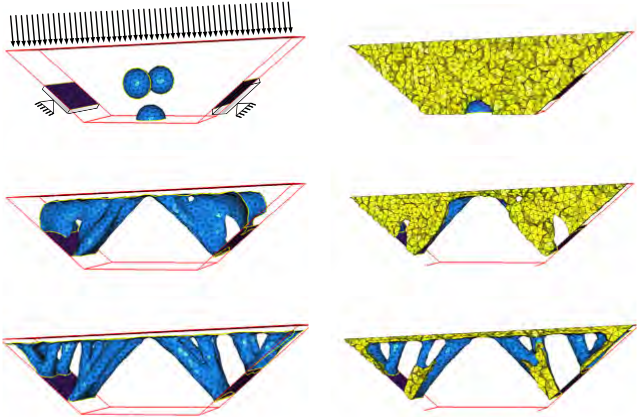
Figure 9.11: (From top to bottom) Initial (with boundary conditions), 30 th and final (70 th ) iterations of the 3d optimal bridge test case.
