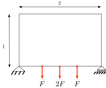
Figure 4.20: Boundary conditions for the 3-force bridge.
