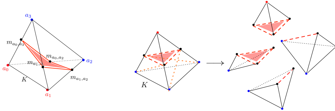
Figure 8.39: ( Left ) One of the possible situations when \mathcal{S}_{\phi_{\mathcal{T}}} (in light red) crosses an element K \in \mathcal{T} ; ( right ) splitting pattern for a tetrahedron K \in \mathcal{T} which is crossed by \mathcal{S}_{\phi_{\mathcal{T}}} in such a way as three of its vertices share the same sign (the blue ones).
