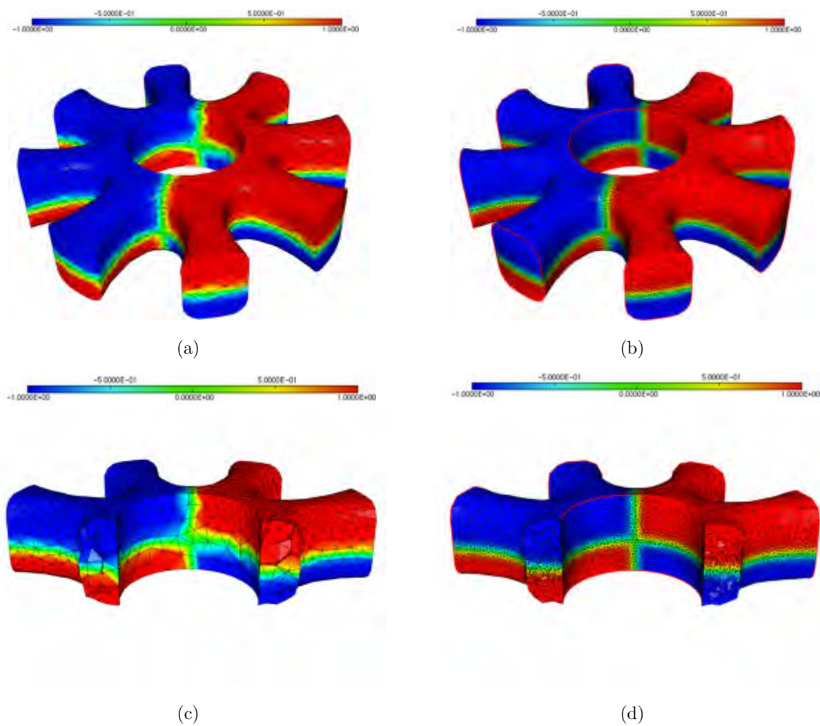
Figure 8.36: Remeshing with respect to a size map devised for the control of the interpolation error of function f defined by (8.72). (a) The initial mesh \mathcal{T} , together with the isolines of f , (c) a cut in the mesh; (b) the resulting mesh \tilde{\mathcal{T}} , with the isolines of f , (d) a cut in \tilde{\mathcal{T}} .
