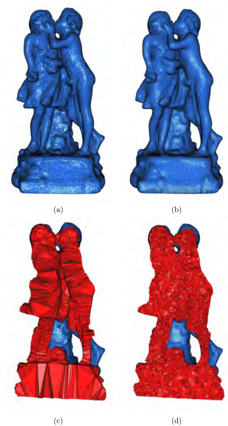
Figure 8.35: Remeshing of the pbscu model, enclosed in a box of dimensions 304 \times 574 \times 190 . The parameters used for the computation are: h_{min} = 1 , h_{max} = 50 , h_{grad} = 1.2 and \varepsilon = 1 . (a)-(c) Initial mesh \mathcal{T} ; (b)-(d) final result \tilde{\mathcal{T}} .
