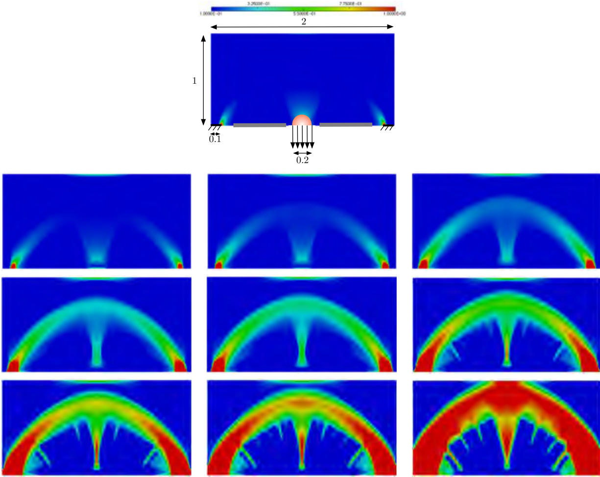
Figure 5.3: Minimization of the compliance with uncertainties over the body forces; from left to right, top to bottom, m = 0 (with boundary conditions), 0.05, 0.1, 0.2, 0.35, 0.5, 1, 1.5, 2, 5.
