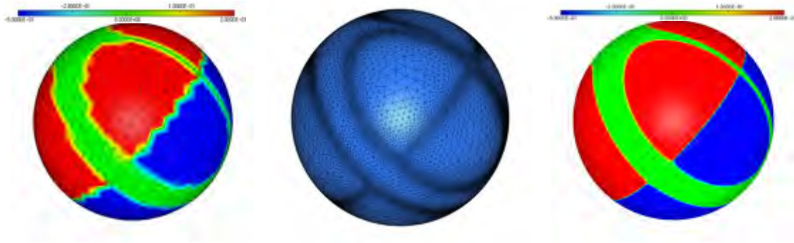
Figure 8.16: (left) Initial triangulation \mathcal{S} , with the isolines of the linear interpolate of f over \mathcal{S} ; (middle) resulting triangulation after 5 remeshing procedures; (right) isolines of the linear interpolate of f over the resulting triangulation.
