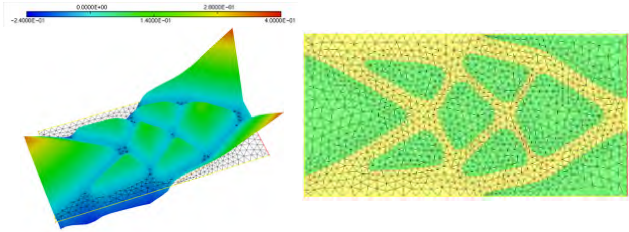
Figure 9.1: (Left) graph of a level set function \phi associated to a shape \Omega ; (right) a corresponding meshed description: the whole computational box D is equipped with a mesh \mathcal{T}_\Omega (composed of the yellow and green elements), and the submesh \mathcal{T}'_\Omega is composed of the yellow triangles.
