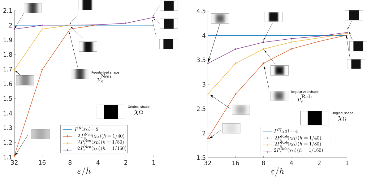
FIGURE 4. Convergence of the quantities (left) 2P_\varepsilon^{\text{Neu}}(\chi_\Omega) and (right) 2P_\varepsilon^{\text{Rob}}(\chi_\Omega) to the exact values of the relative and total perimeters \text{Per}^R(\Omega) and \text{Per}^T(\Omega) in the numerical validation example of Section 6.1 .
