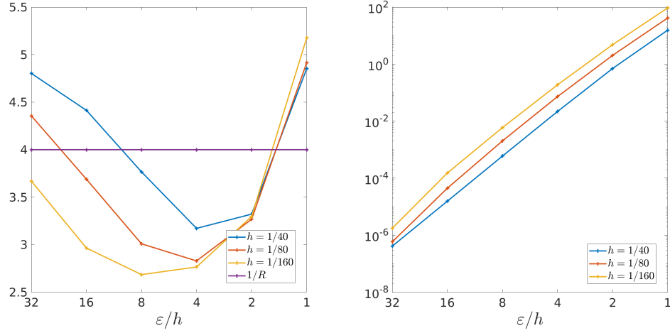
FIGURE 10. (Left) mean value m_\epsilon over \partial\Omega of the derivative 2g_{u,\epsilon} of the approximate perimeter functional P_\epsilon^{\text{Rob}}(u) ; (right) variance \sigma_\epsilon over \partial\Omega of this derivative in the example of Section 6.2.2.
