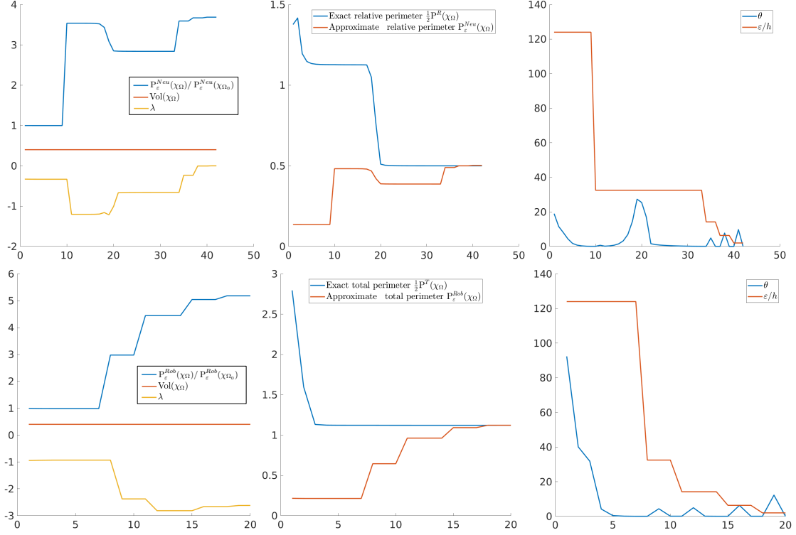
FIGURE 12. Evolution of the quantities involved in the (upper row) relative and (lower row) total perimeter minimization problem under volume constraint of Section 6.3 . The values of the perimeter (normalized with that of the initial design), volume and Lagrange multiplier are represented on the left column; the exact relative and total perimeters \text{Per}^R(\Omega) or \text{Per}^T(\Omega) of the shape \Omega are compared with the approximate values P_\varepsilon^{\text{Neu}}(\chi_\Omega) and P_\varepsilon^{\text{Rob}}(\chi_\Omega) through the iterations in the central column, and the algorithm parameters \theta and \varepsilon/h are represented on the right column.
