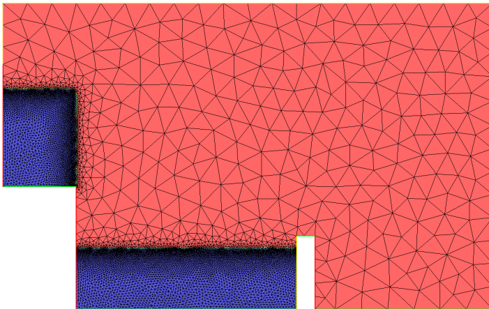
Evolution of a collapsing water column
